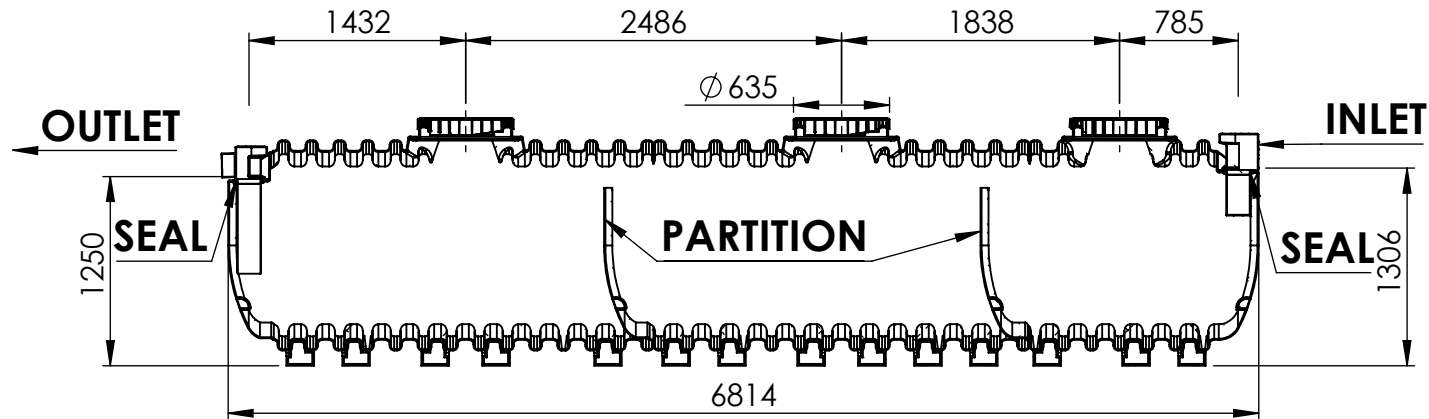
SECTION F-F SCALE 1 : 50
